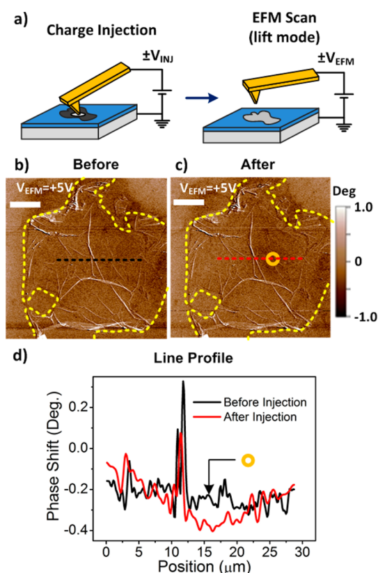
Figure 1. Charge injection experiments on pristine GO. (a) Schematic of the EFM charge injection. Charge injection ( V_{INJ} = +10 V) is performed with the conducting tip and the charge propagation is observed using EFM lift mode with tip voltage V_{EFM} . (b) Initial charge state for V_{EFM} = +5 V. Yellow dashed line indicate outer edge of the GO flake. (c) EFM charge state after positive charge injection to the yellow circled point on GO flake for V_{EFM} = +5 V. (d) The line profile to the EFM images of before and after charge injection shows that the charge injection to the GO flake is not efficient. All scale bars in (b) and (c) are 10 \mu m .
